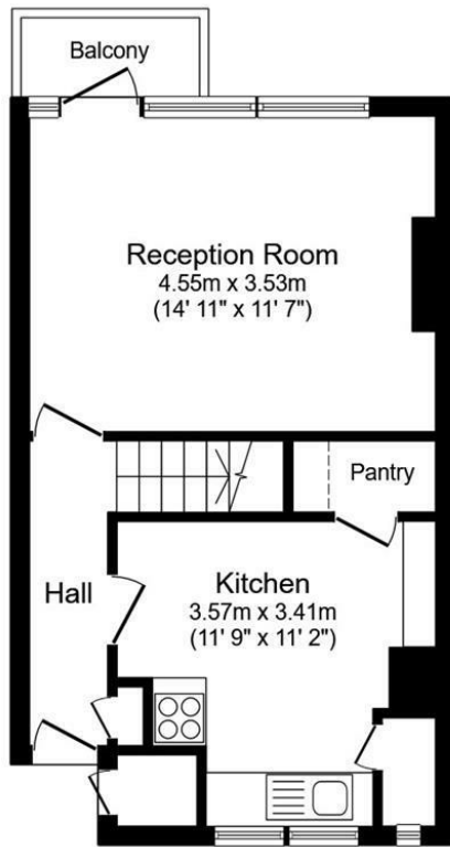
Second Floor Floor area 35.2 sq.m. (379 sq.ft.)
